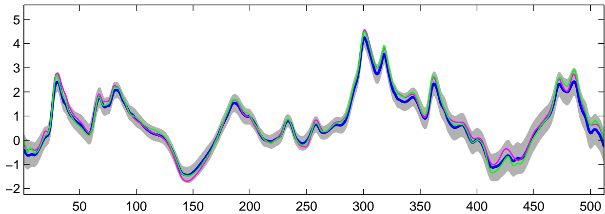
Estimated C_0(t) using G-WFMM: DE data, run 5
