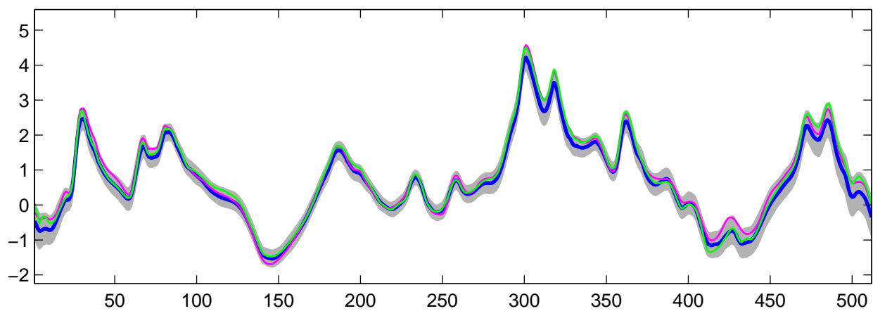
Estimated C_0(t) using R-WFMM: DE data, run 5
