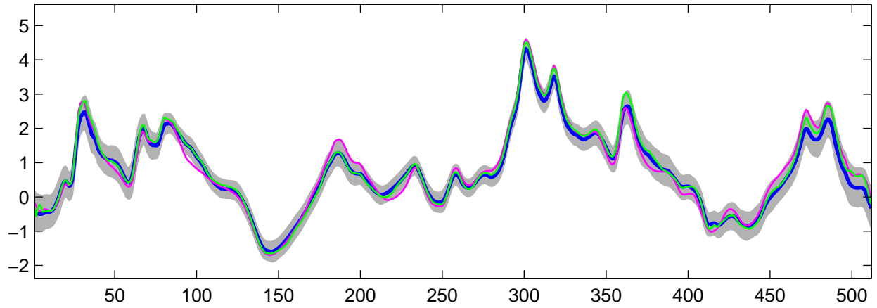
Estimated C_0(t) using G-WFMM: Normal data, run 5
