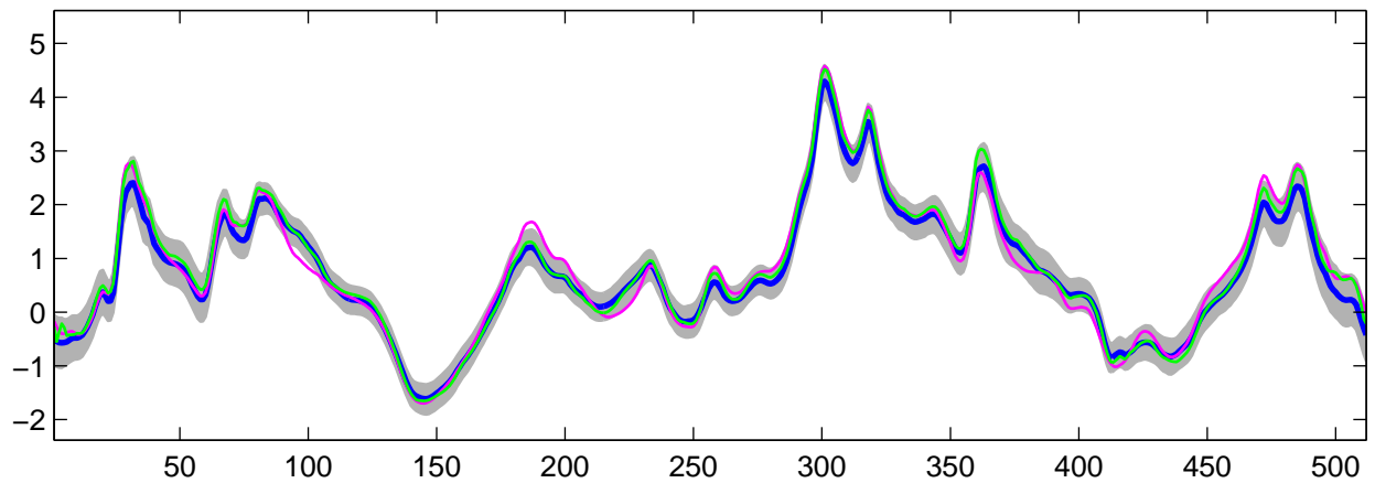
Estimated C_0(t) using R-WFMM: Normal data, run 5
