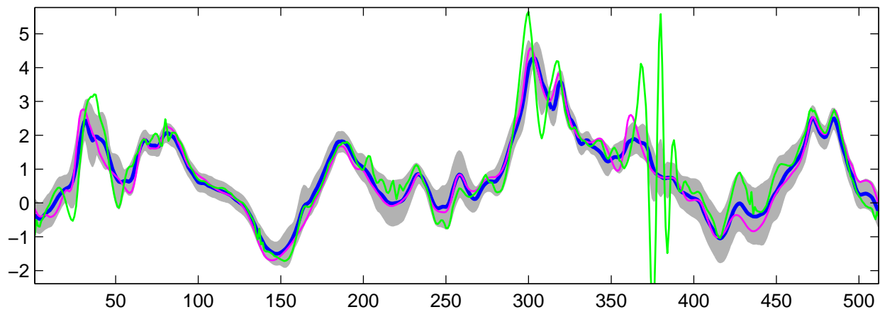
Estimated C_0(t) using G-WFMM: t_1 data, run 5
