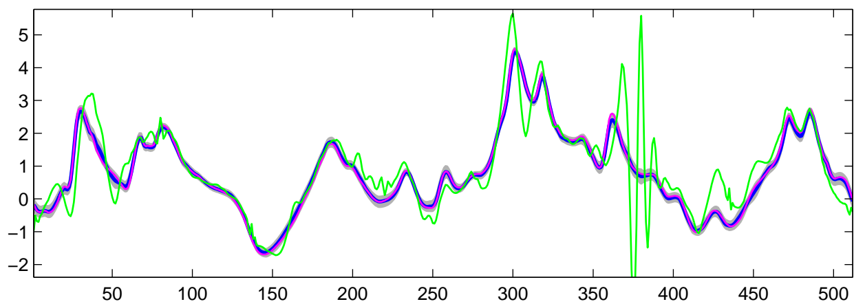
Estimated C_0(t) using R-WFMM: t_1 data, run 5
