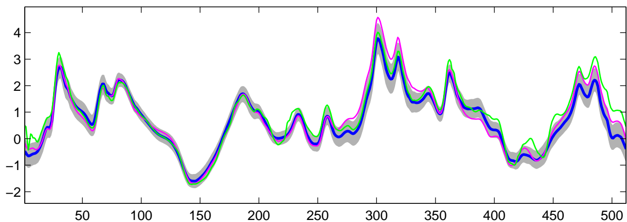
Estimated C_0(t) using R-WFMM: t_2 data, run 5
