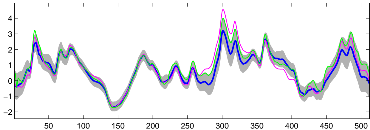
Estimated C_0(t) using G-WFMM: t_2 data, run 5
