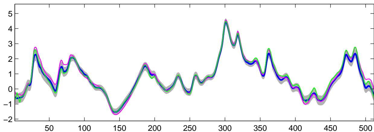
Estimated C_0(t) using R-WFMM: t_3 data, run 5
