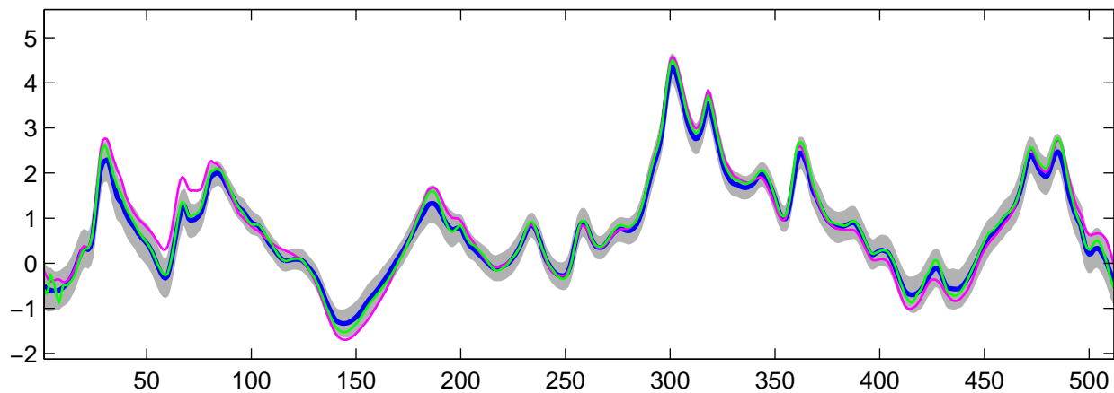
Estimated C_0(t) using G-WFMM: t_3 data, run 5
