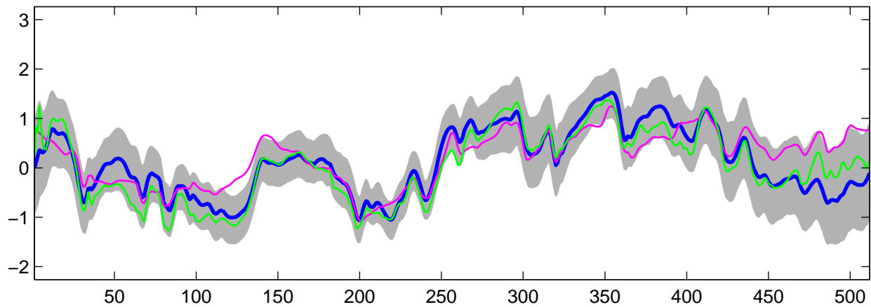
Estimated C_1(t) using R-WFMM: DE data, run 5
