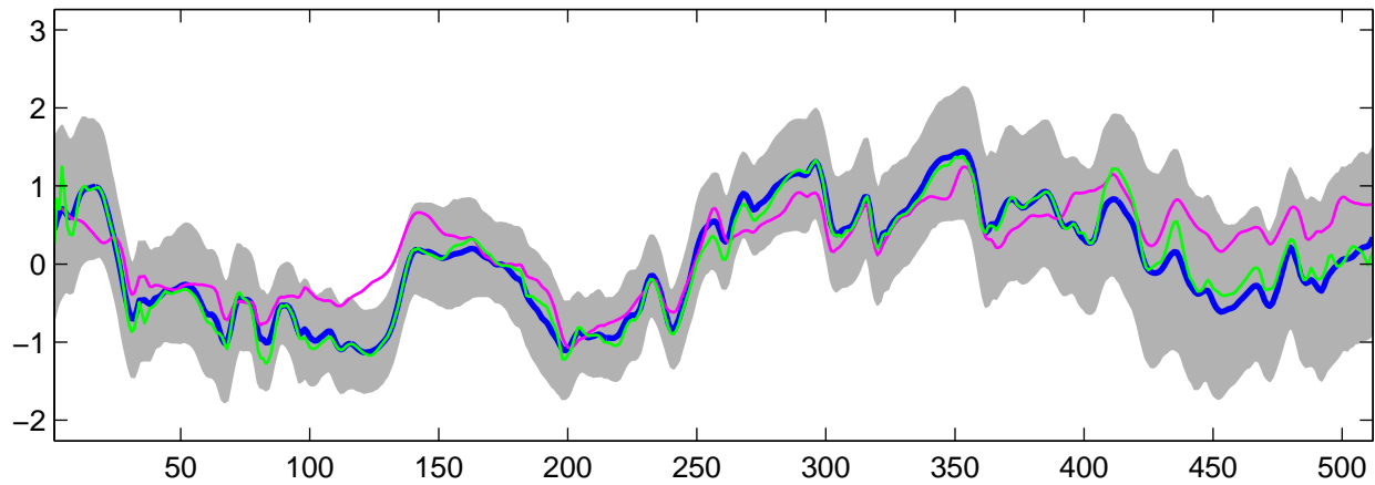
Estimated C_1(t) using G-WFMM: DE data, run 5
