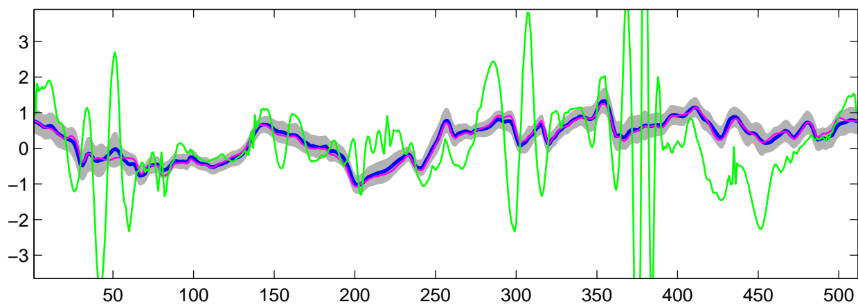
Estimated C_1(t) using R-WFMM: t_1 data, run 5
