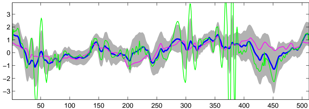
Estimated C_1(t) using G-WFMM: t_1 data, run 5
