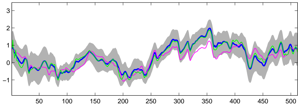
Estimated C_1(t) using G-WFMM: t_3 data, run 5
