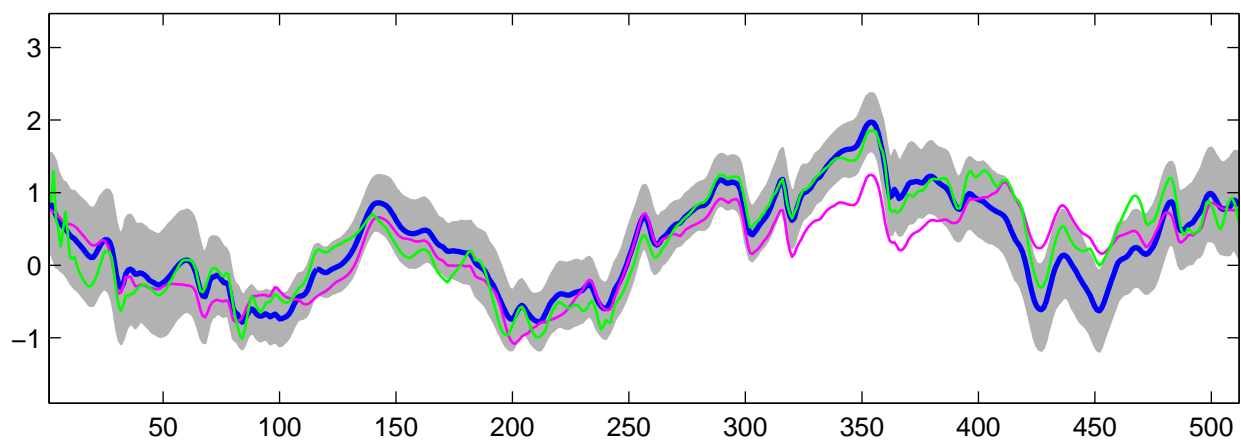
Estimated C_1(t) using R-WFMM: t_3 data, run 5
