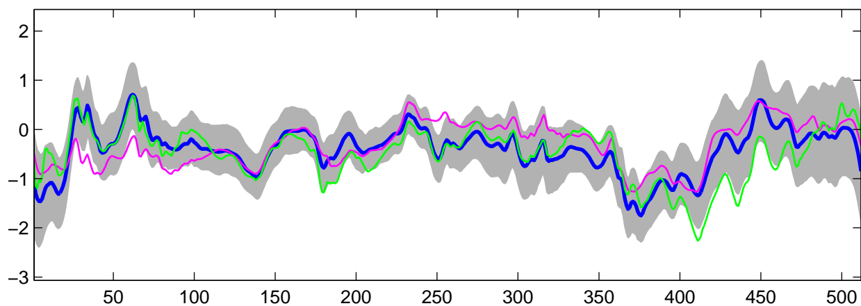
Estimated C_2(t) using R-WFMM: DE data, run 5
