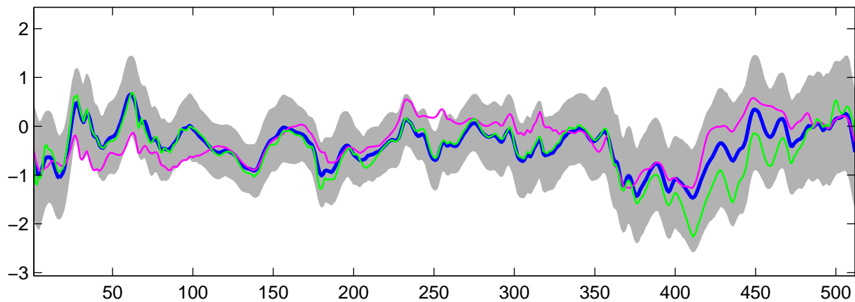
Estimated C_2(t) using G-WFMM: DE data, run 5
