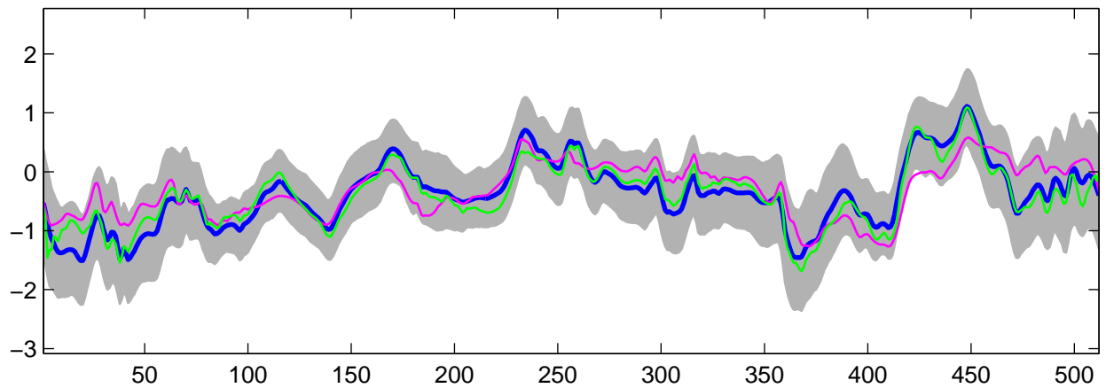
Estimated C_2(t) using R-WFMM: Normal data, run 5
