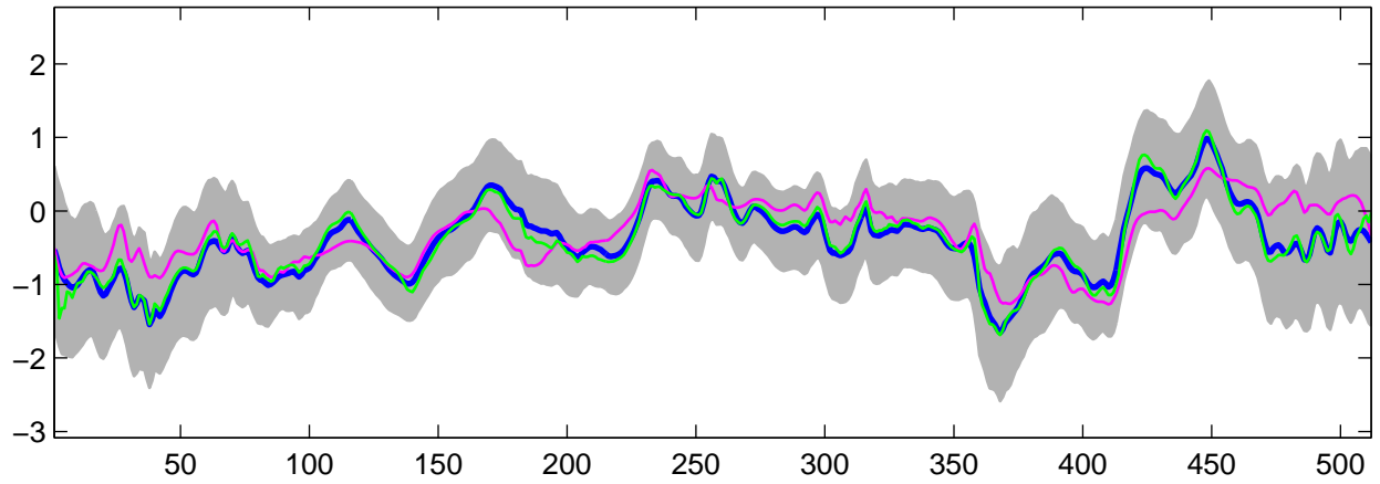
Estimated C_2(t) using G-WFMM: Normal data, run 5
