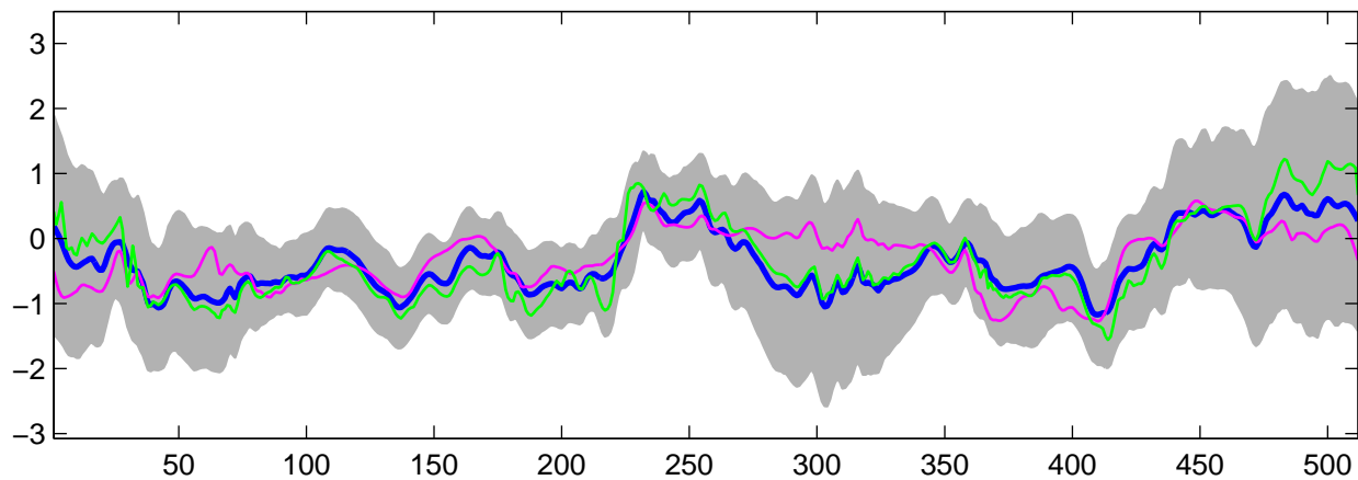
Estimated C_2(t) using G-WFMM: t_2 data, run 5
