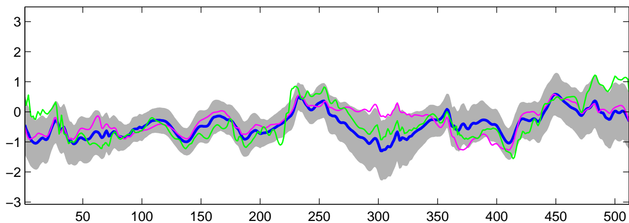
Estimated C_2(t) using R-WFMM: t_2 data, run 5
