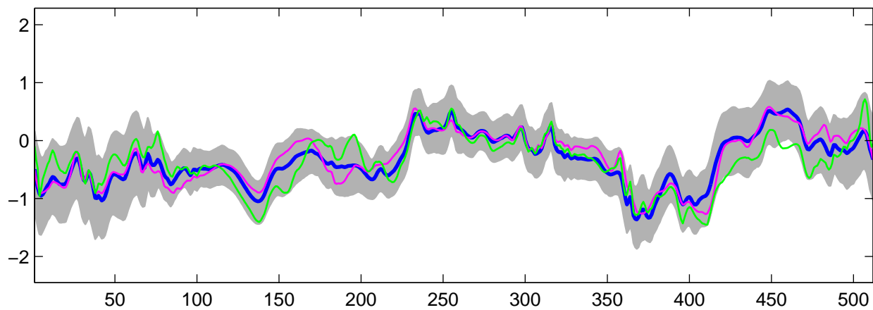
Estimated C_2(t) using R-WFMM: t_3 data, run 5
