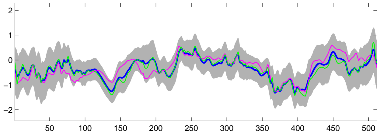
Estimated C_2(t) using G-WFMM: t_3 data, run 5
