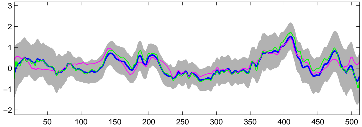
Estimated C_3(t) using G-WFMM: Normal data, run 5
