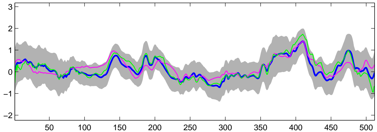
Estimated C_3(t) using R-WFMM: Normal data, run 5
