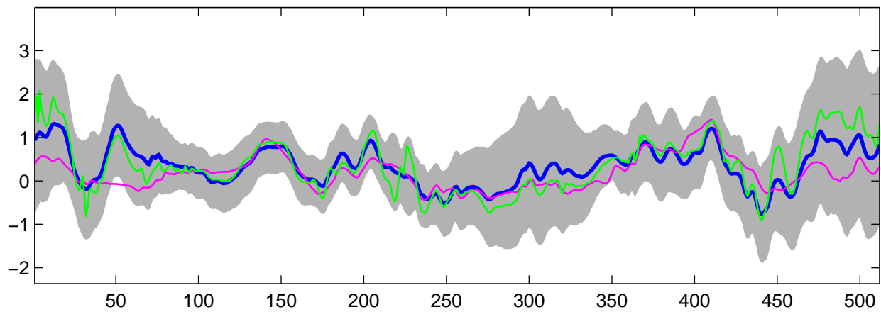
Estimated C_3(t) using G-WFMM: t_2 data, run 5
