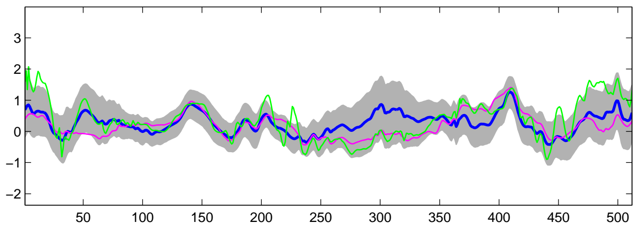
Estimated C_3(t) using R-WFMM: t_2 data, run 5
