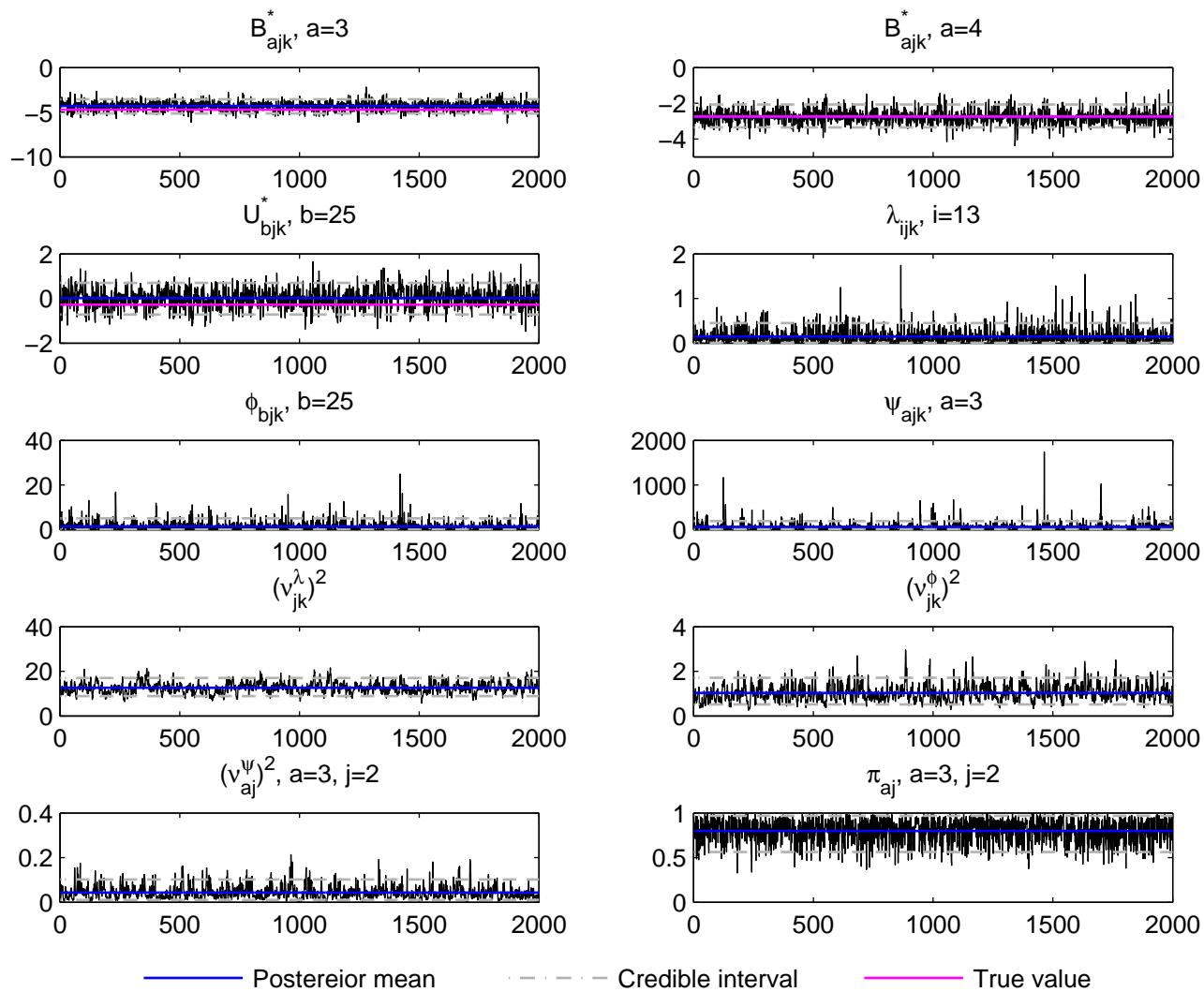
Trace plot, j=2, k=2 , DE data, simulation run 5
