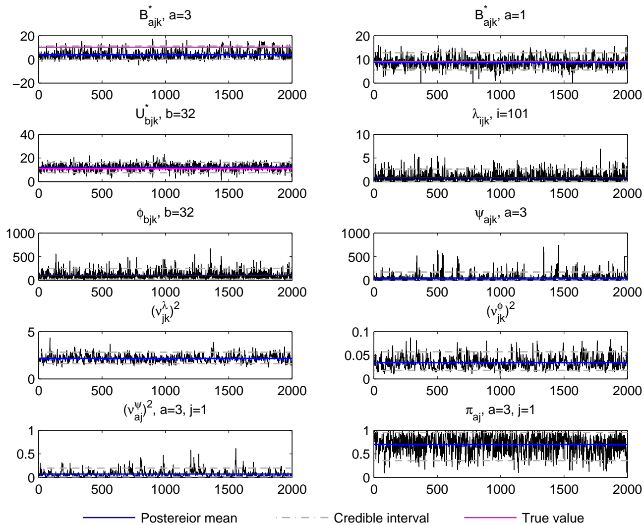
Trace plot, j=1, k=5 , Normal data, simulation run 5
