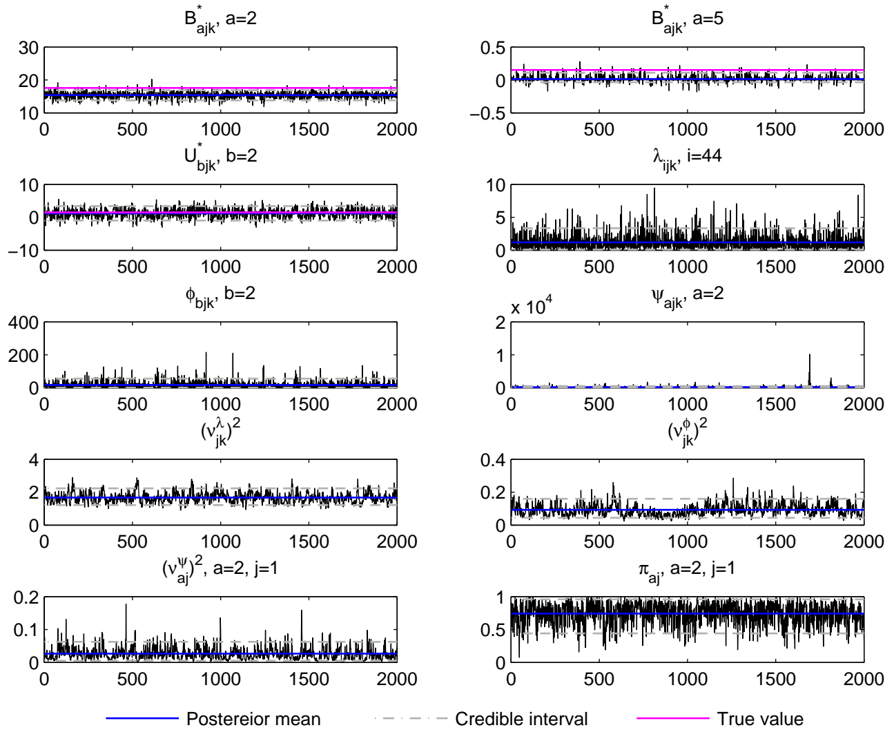
Trace plot, j=1, k=2, t_2 data, simulation run 5
