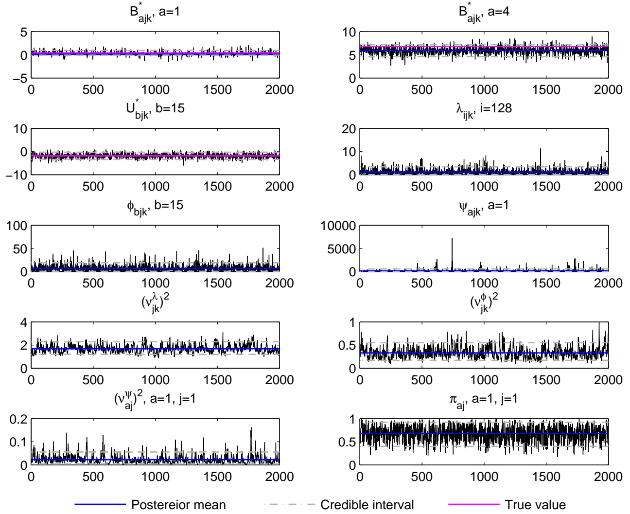
Trace plot, j=1, k=6, t_3 data, simulation run 5
