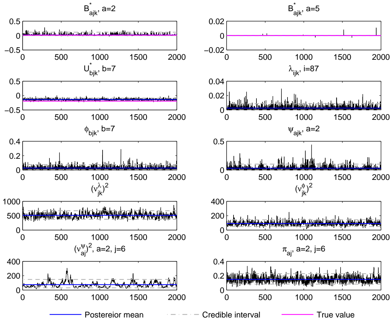
Trace plot, j=6, k=2 , DE data, simulation run 5
