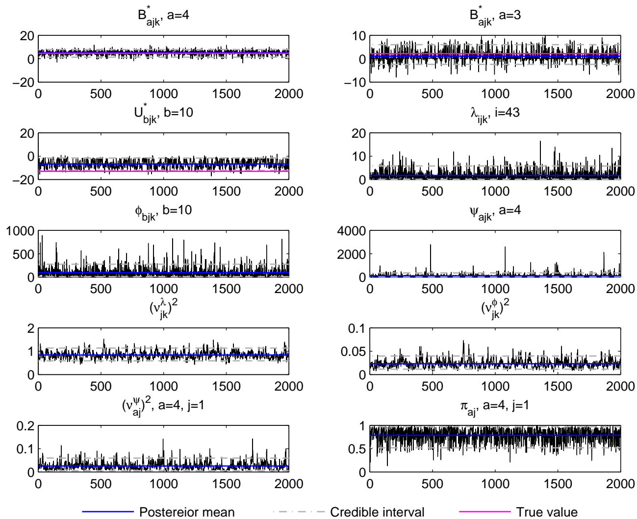
Trace plot, j=1, k=4 , Normal data, simulation run 5
