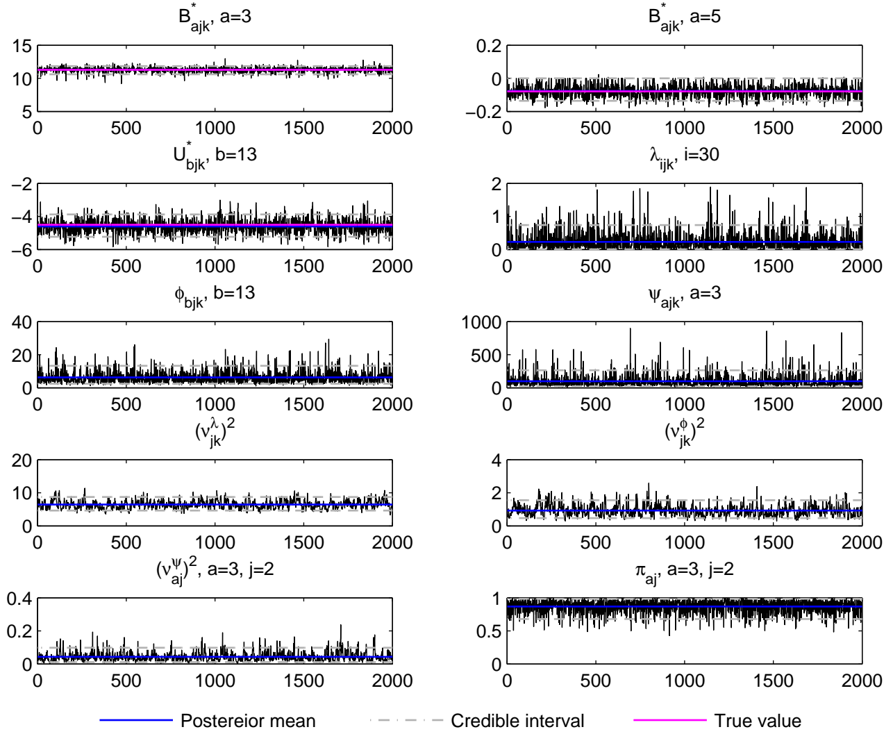
Trace plot, j=2, k=3, t_i data, simulation run 5
