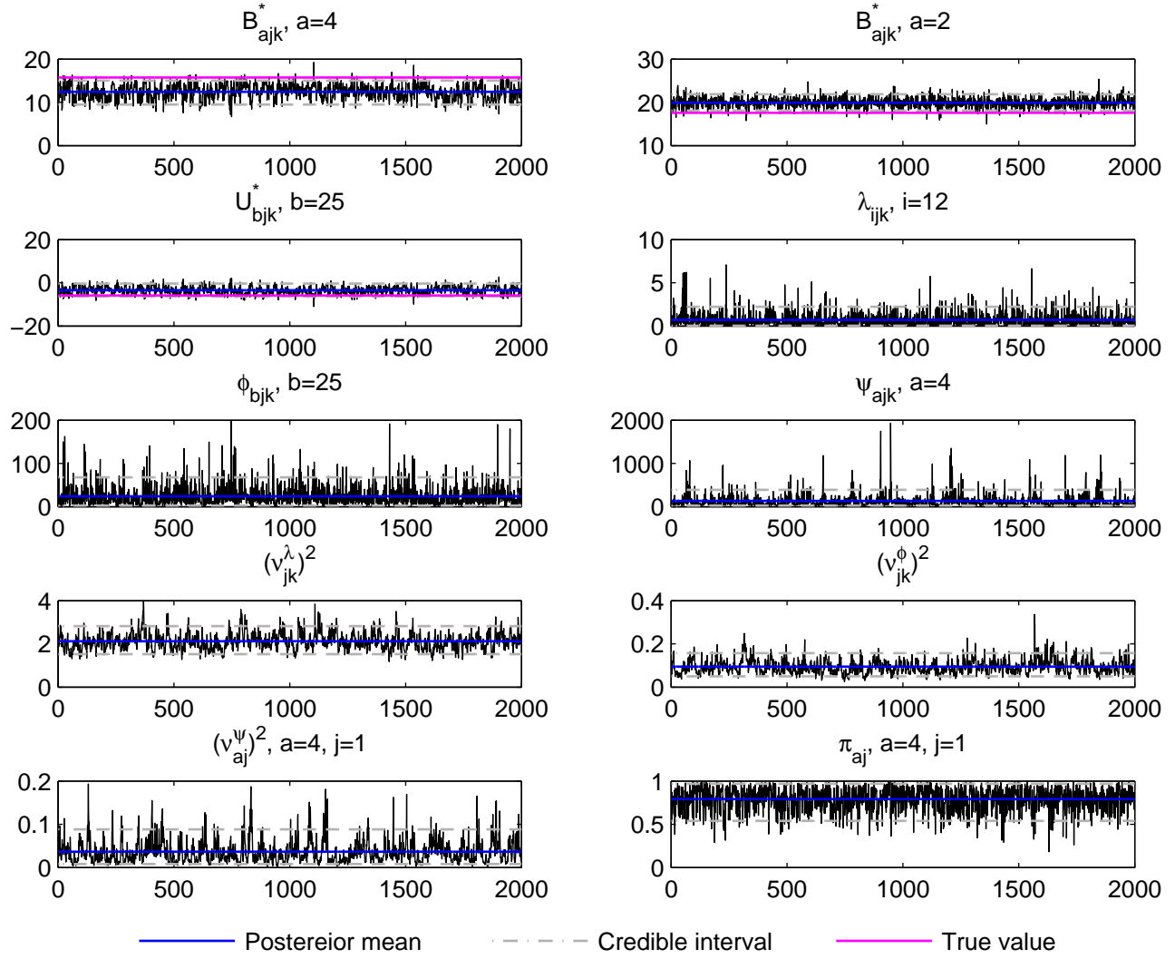
Trace plot, j=1, k=2, t_3 data, simulation run 5
