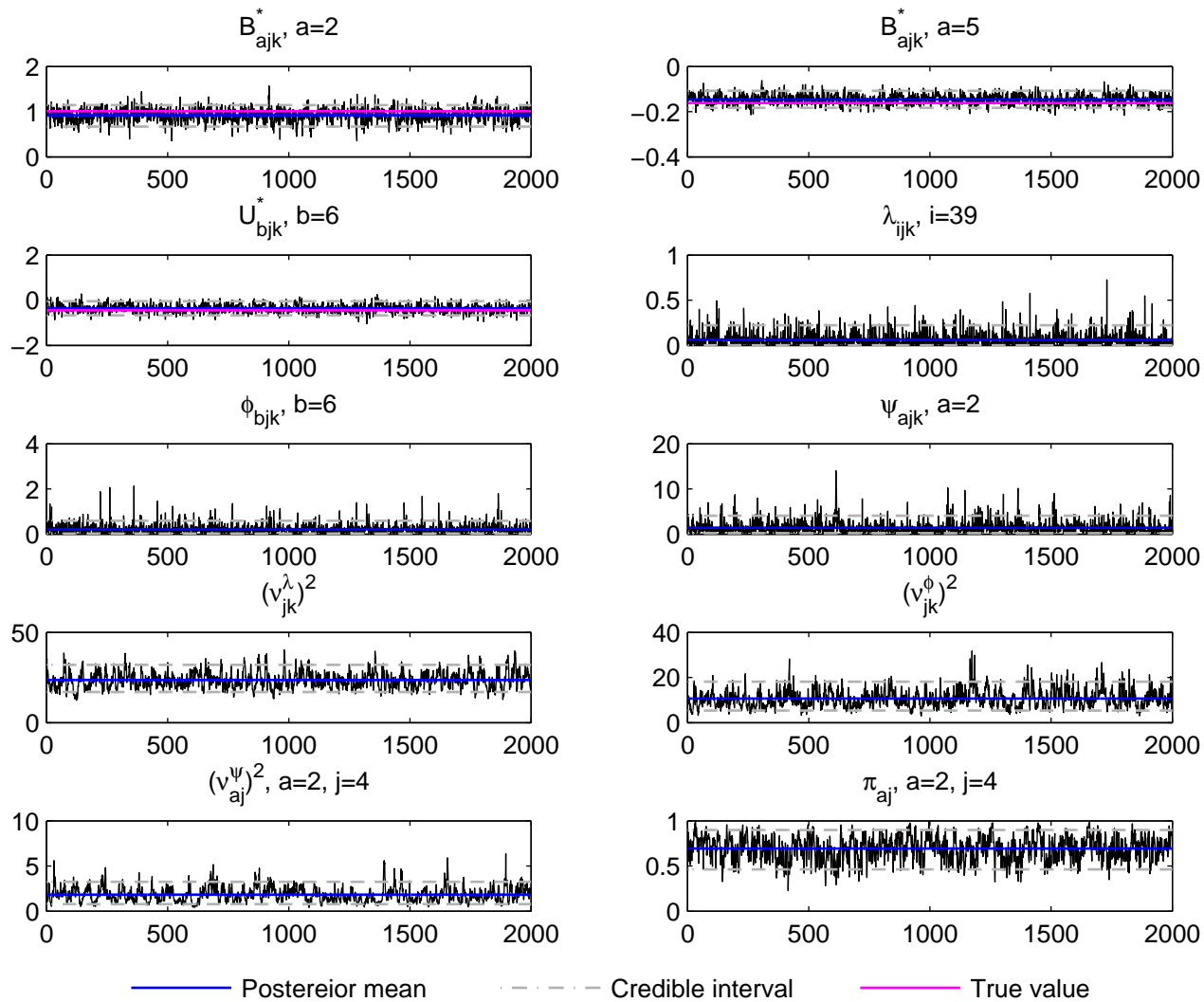
Trace plot, j=4, k=3 , DE data, simulation run 5
