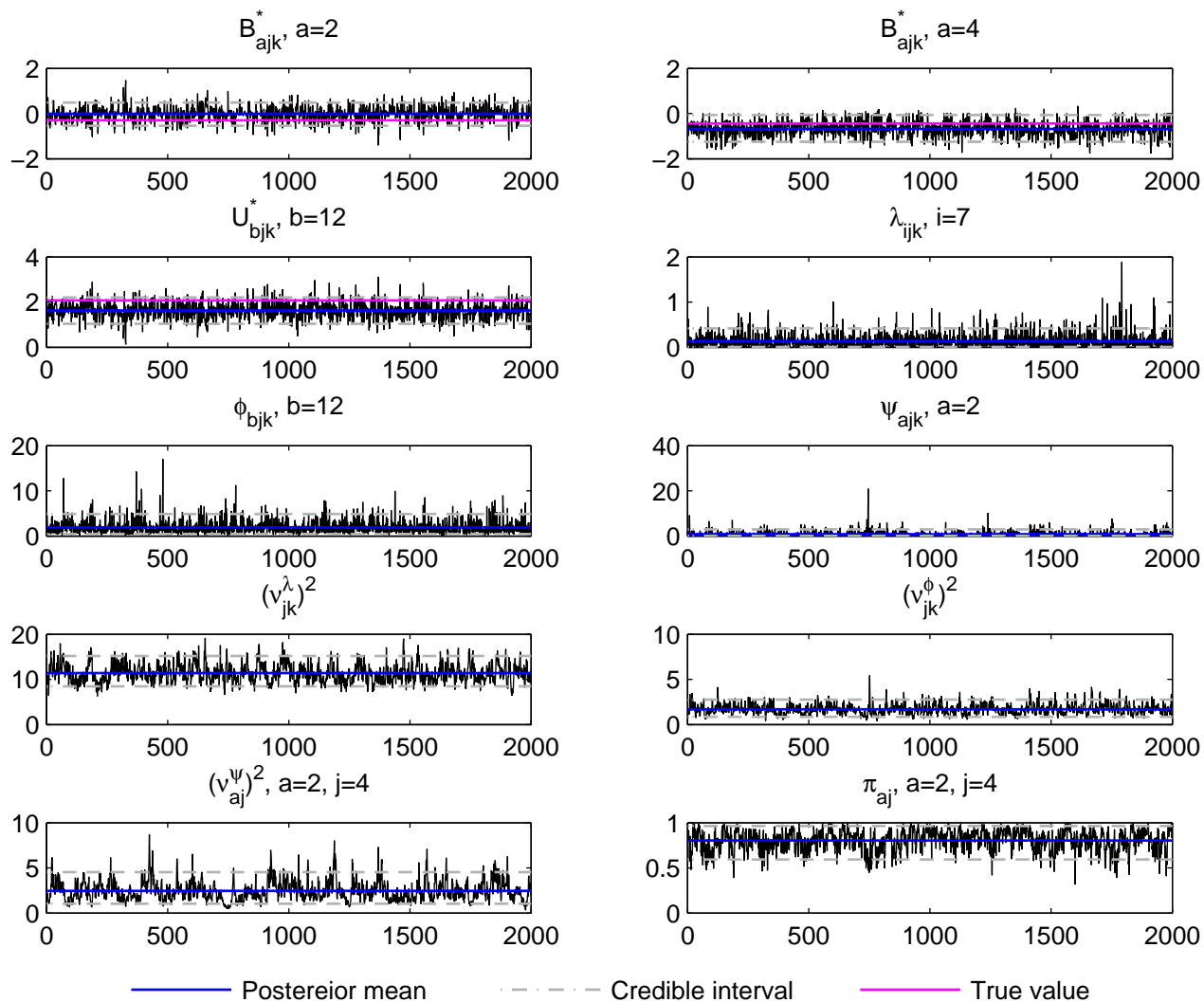
Trace plot, j=4, k=1 , Normal data, simulation run 5
