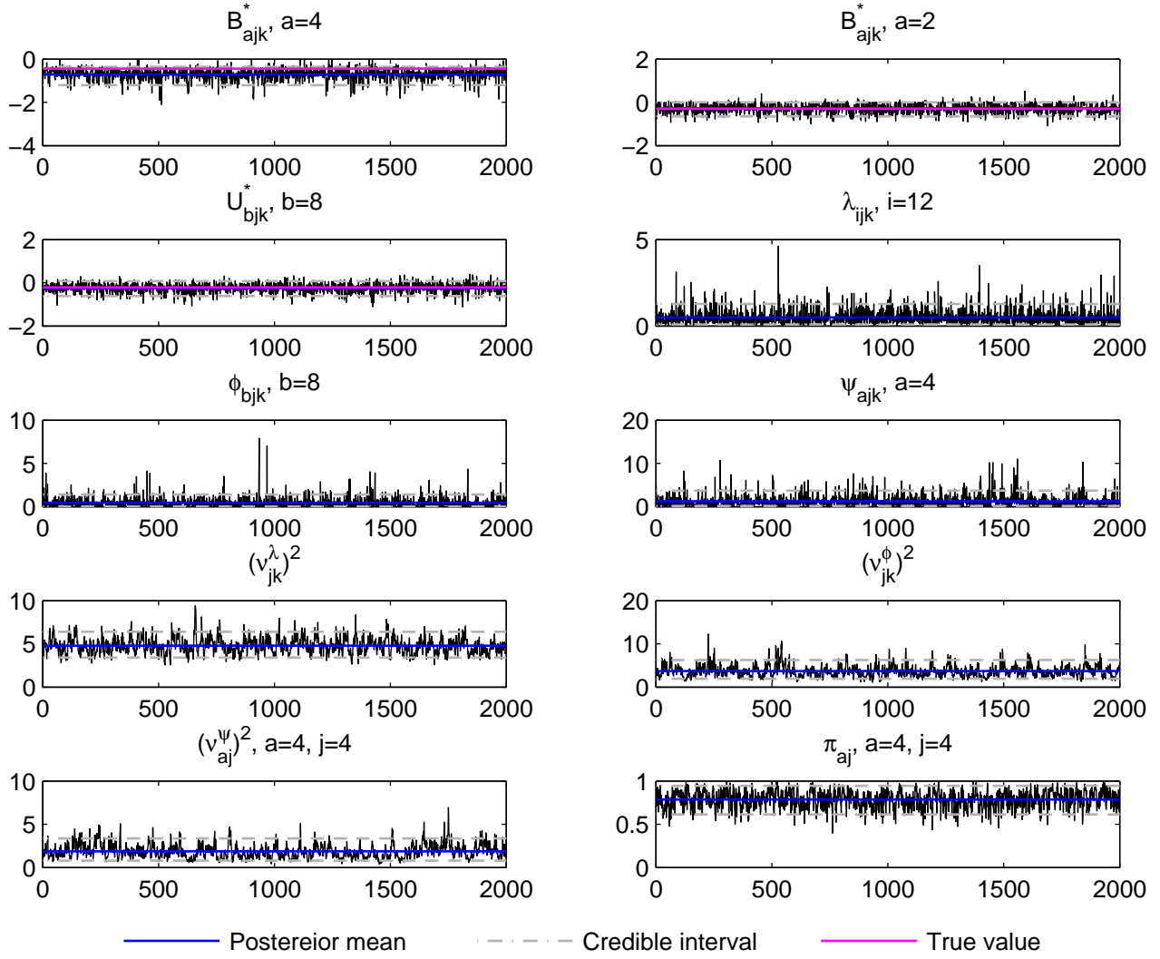
Trace plot, j=4, k=1, t_j data, simulation run 5
