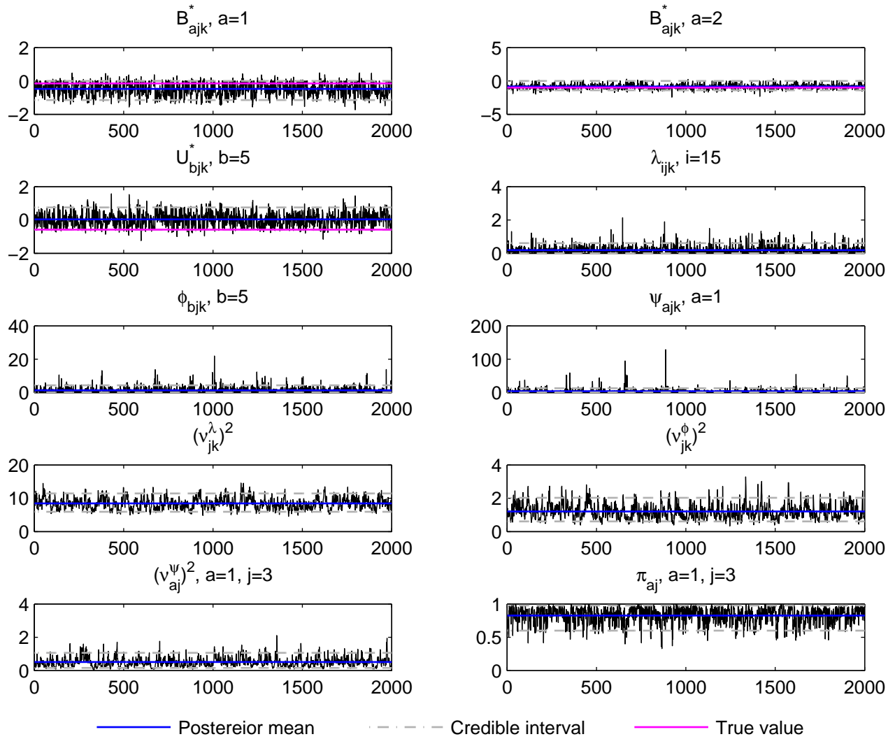
Trace plot, j=3, k=6, t_2 data, simulation run 5
