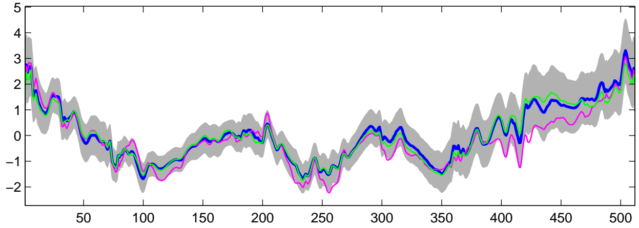
Estimated U_{10}(t) using G-WFMM: DE data, run 5
