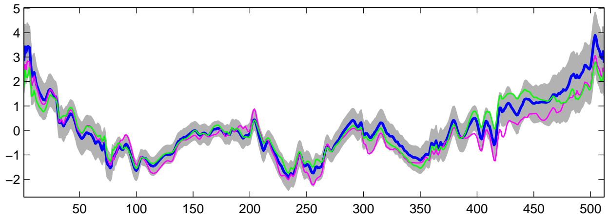
Estimated U_{10}(t) using R-WFMM: DE data, run 5
