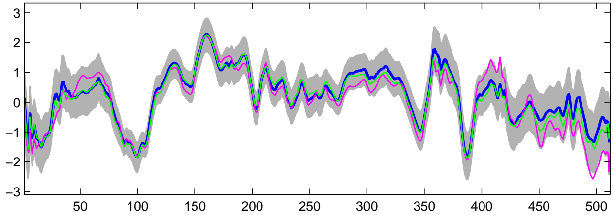
Estimated U_{10}(t) using G-WFMM: Normal data, run 5
