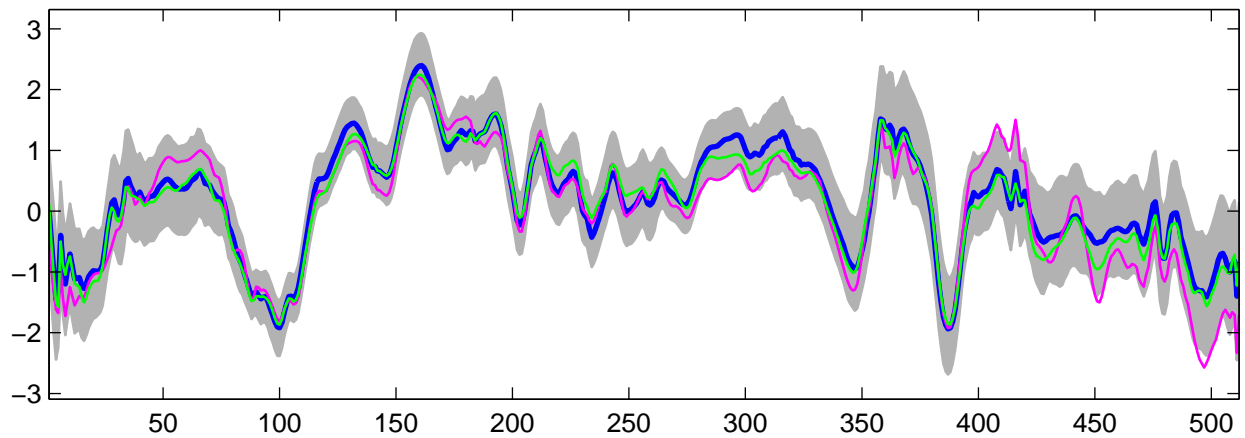
Estimated U_{10}(t) using R-WFMM: Normal data, run 5
