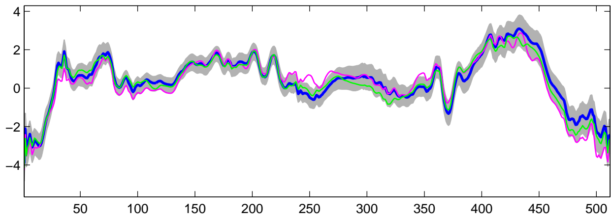
Estimated U_{11}(t) using R-WFMM: DE data, run 5
