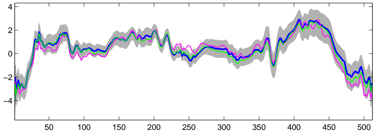
Estimated U_{11}(t) using G-WFMM: DE data, run 5
