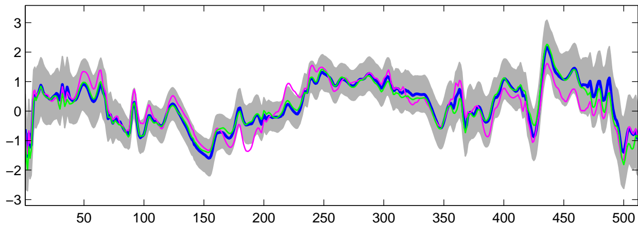
Estimated U_{11}(t) using G-WFMM: Normal data, run 5
