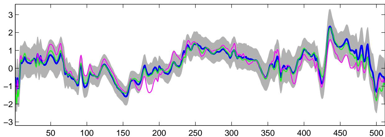
Estimated U_{11}(t) using R-WFMM: Normal data, run 5
