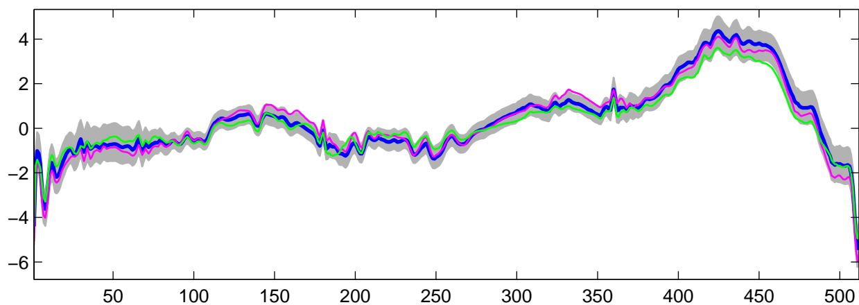
Estimated U_{11}(t) using R-WFMM: t_3 data, run 5
