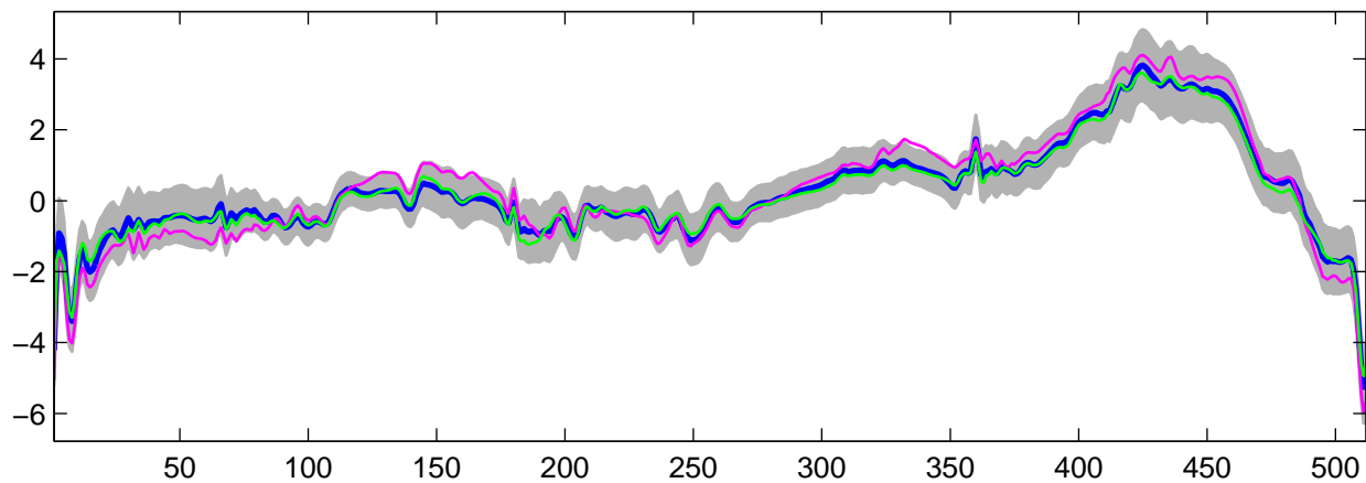
Estimated U_{11}(t) using G-WFMM: t_3 data, run 5
