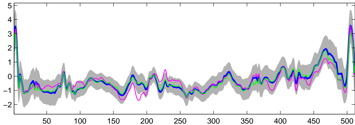
Estimated U_{12}(t) using G-WFMM: Normal data, run 5
