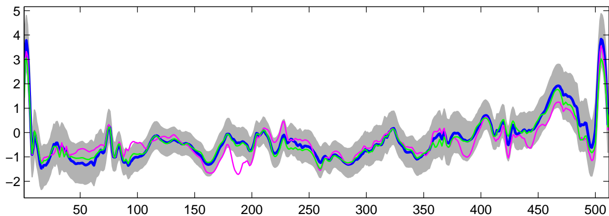
Estimated U_{12}(t) using R-WFMM: Normal data, run 5
