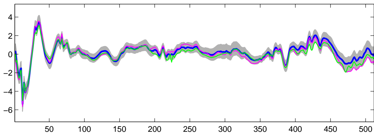
Estimated U_{12}(t) using R-WFMM: t_2 data, run 5
