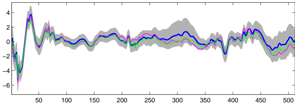
Estimated U_{12}(t) using G-WFMM: t_2 data, run 5
