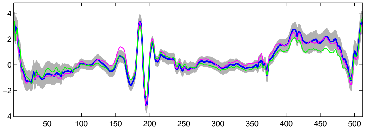
Estimated U_{12}(t) using R-WFMM: t_3 data, run 5
