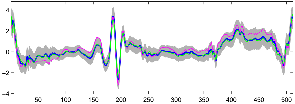
Estimated U_{12}(t) using G-WFMM: t_3 data, run 5
