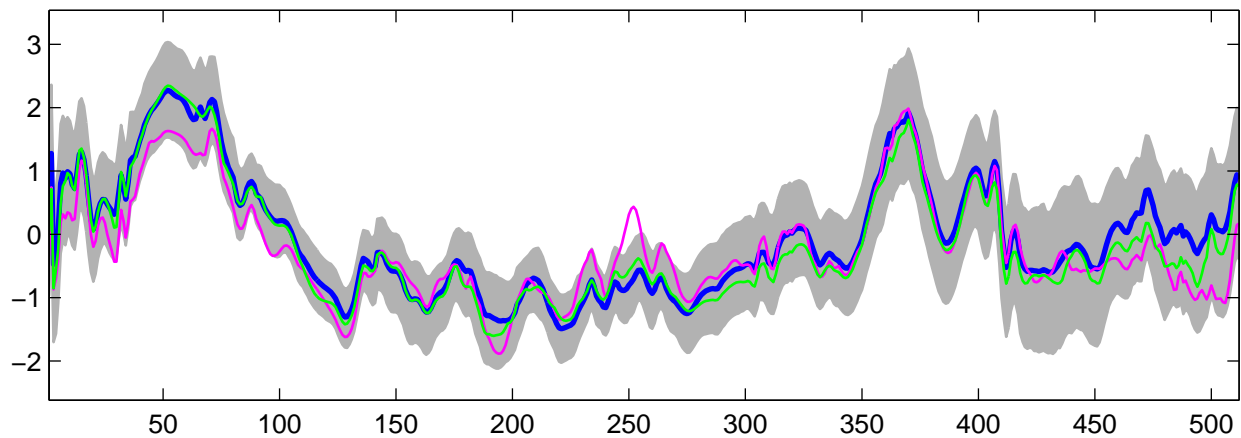
Estimated U_{13}(t) using G-WFMM: DE data, run 5
