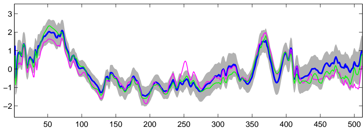
Estimated U_{13}(t) using R-WFMM: DE data, run 5
