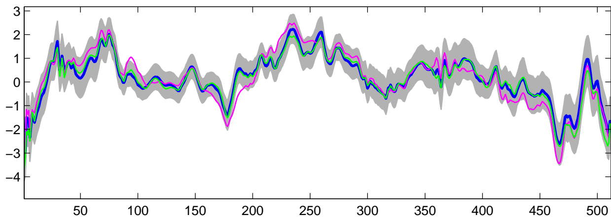
Estimated U_{13}(t) using R-WFMM: Normal data, run 5
