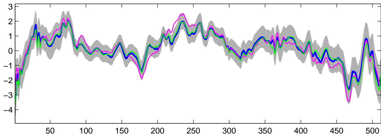
Estimated U_{13}(t) using G-WFMM: Normal data, run 5
