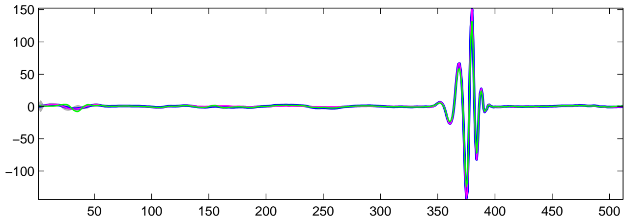
Estimated U_{13}(t) using G-WFMM: t_1 data, run 5
