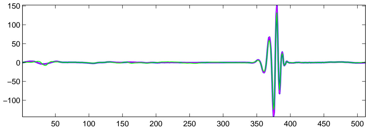
Estimated U_{13}(t) using R-WFMM: t_1 data, run 5
