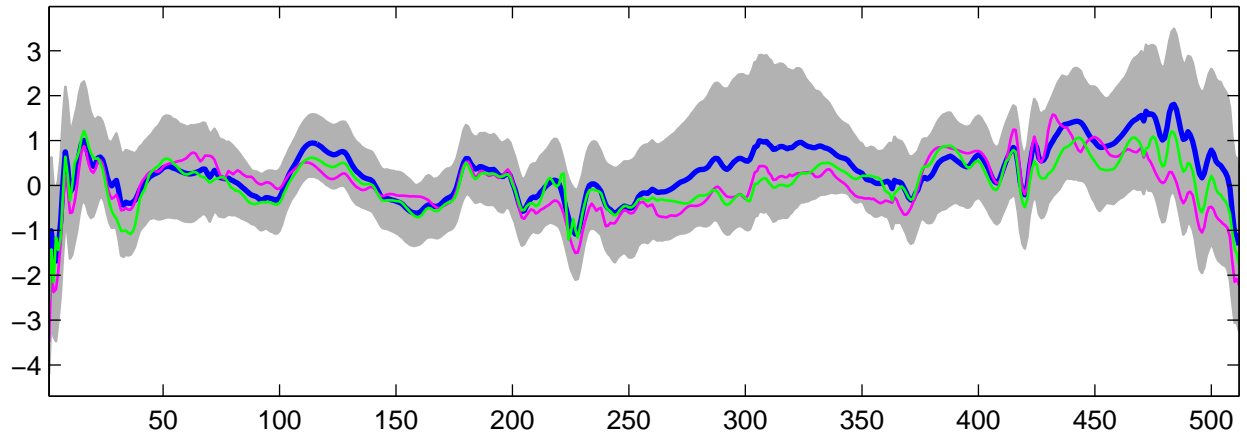
Estimated U_{13}(t) using G-WFMM: t_2 data, run 5
