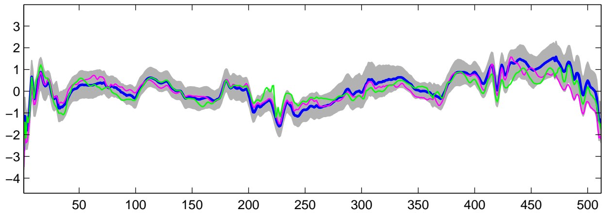
Estimated U_{13}(t) using R-WFMM: t_2 data, run 5
