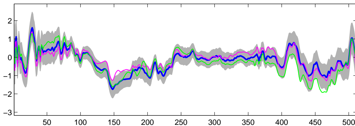
Estimated U_{13}(t) using R-WFMM: t_3 data, run 5
