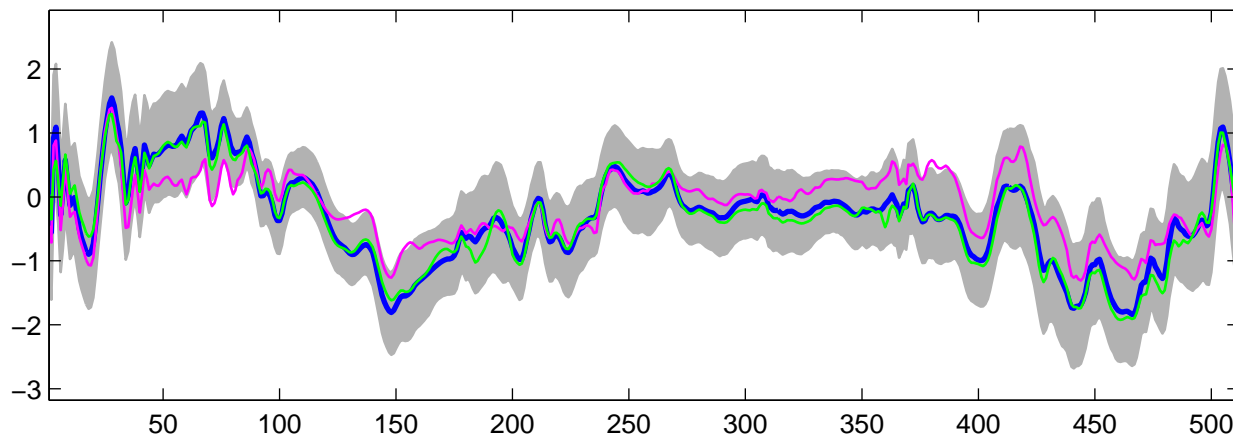
Estimated U_{13}(t) using G-WFMM: t_3 data, run 5
