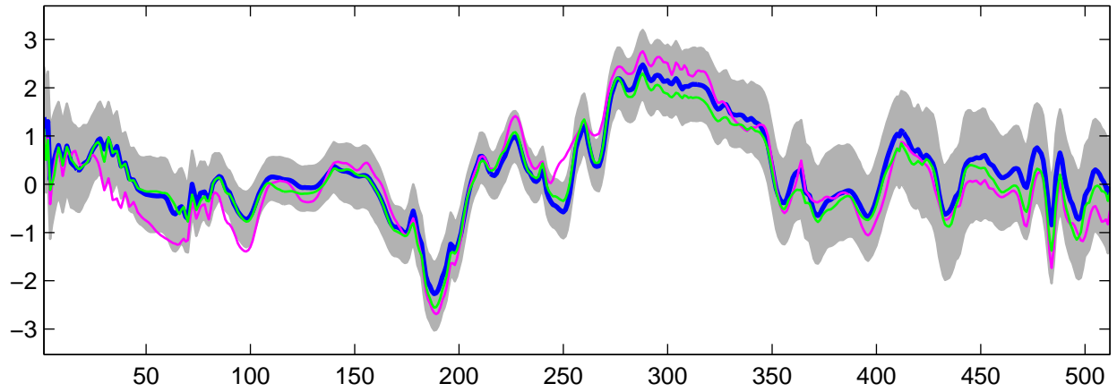
Estimated U_{14}(t) using G-WFMM: DE data, run 5
