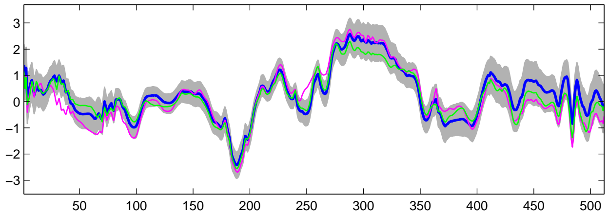
Estimated U_{14}(t) using R-WFMM: DE data, run 5
