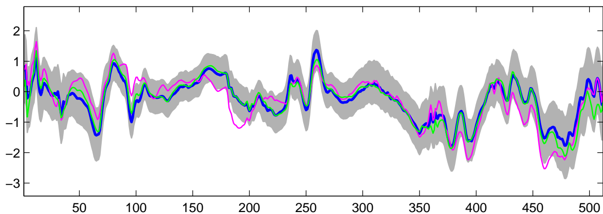
Estimated U_{14}(t) using R-WFMM: Normal data, run 5
