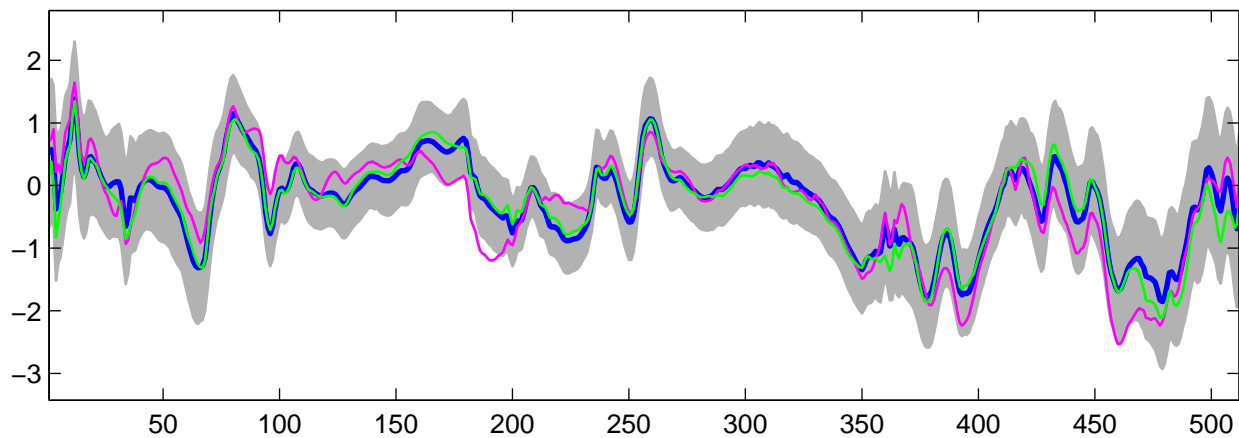
Estimated U_{14}(t) using G-WFMM: Normal data, run 5
