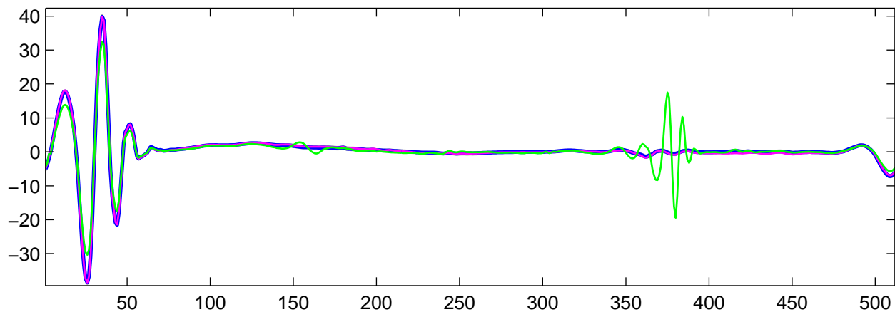
Estimated U_{14}(t) using R-WFMM: t_1 data, run 5
