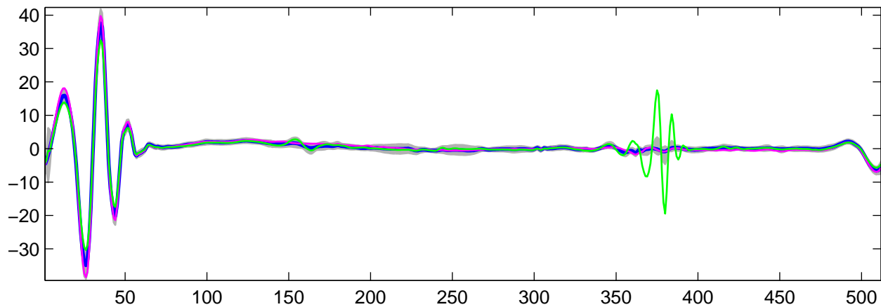
Estimated U_{14}(t) using G-WFMM: t_1 data, run 5
