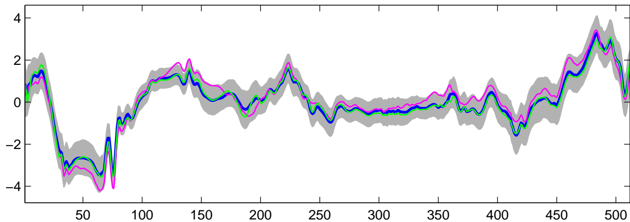
Estimated U_{14}(t) using G-WFMM: t_3 data, run 5
