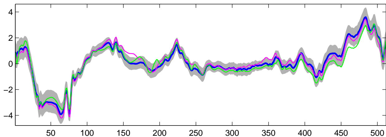
Estimated U_{14}(t) using R-WFMM: t_3 data, run 5
