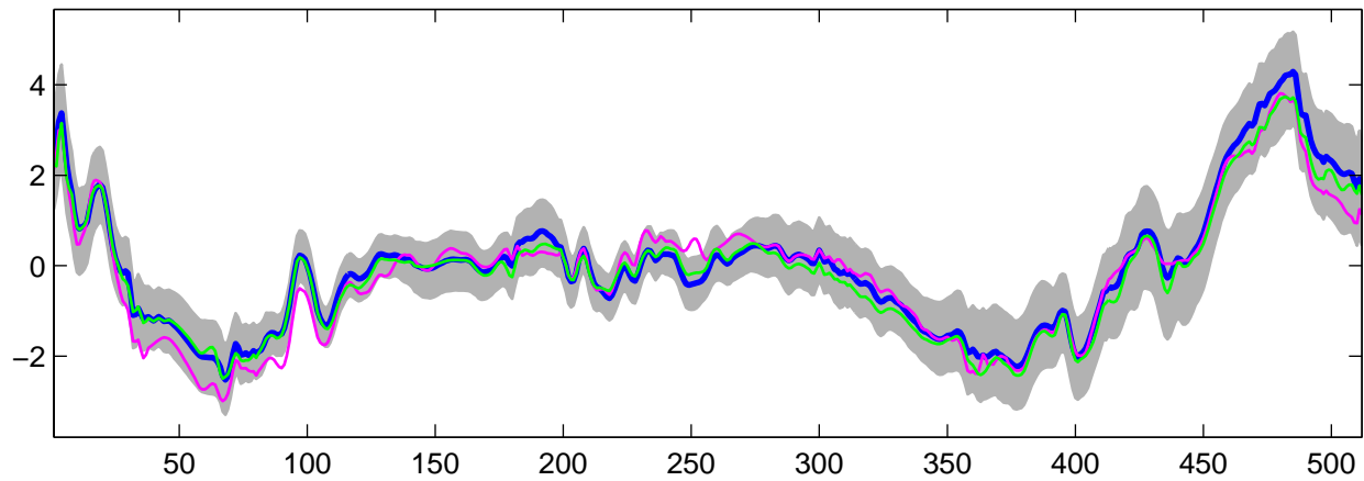
Estimated U_{15}(t) using G-WFMM: DE data, run 5
