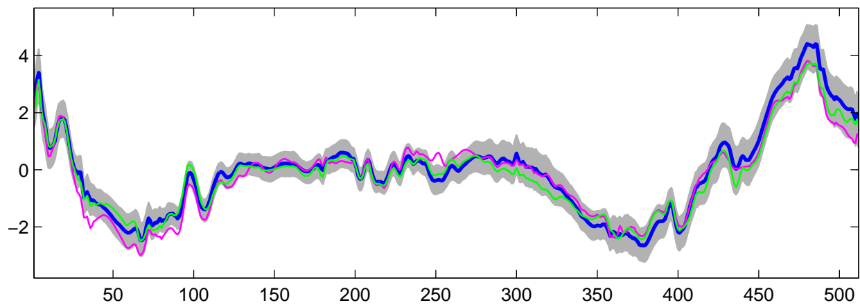
Estimated U_{15}(t) using R-WFMM: DE data, run 5
