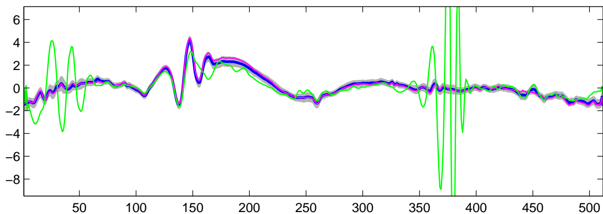
Estimated U_{15}(t) using R-WFMM: t_1 data, run 5
