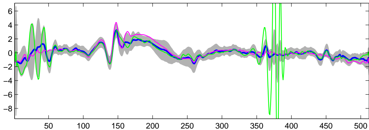
Estimated U_{15}(t) using G-WFMM: t_1 data, run 5
