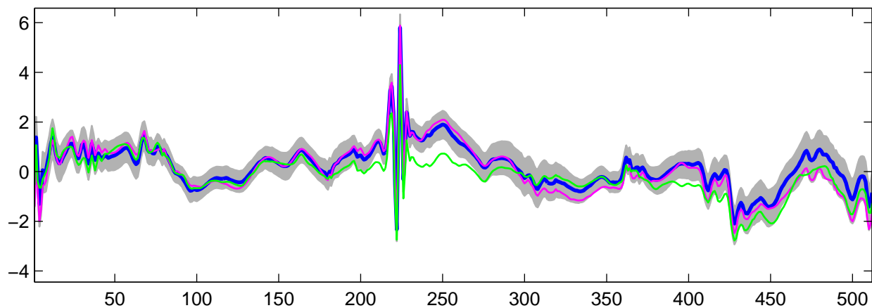
Estimated U_{15}(t) using R-WFMM: t_2 data, run 5
