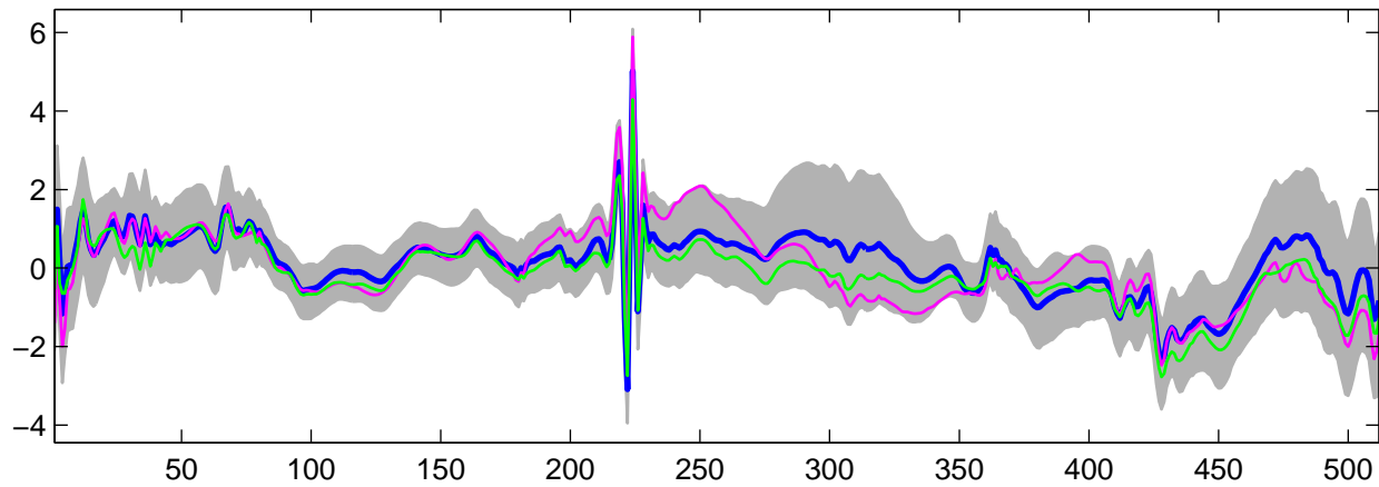
Estimated U_{15}(t) using G-WFMM: t_2 data, run 5
