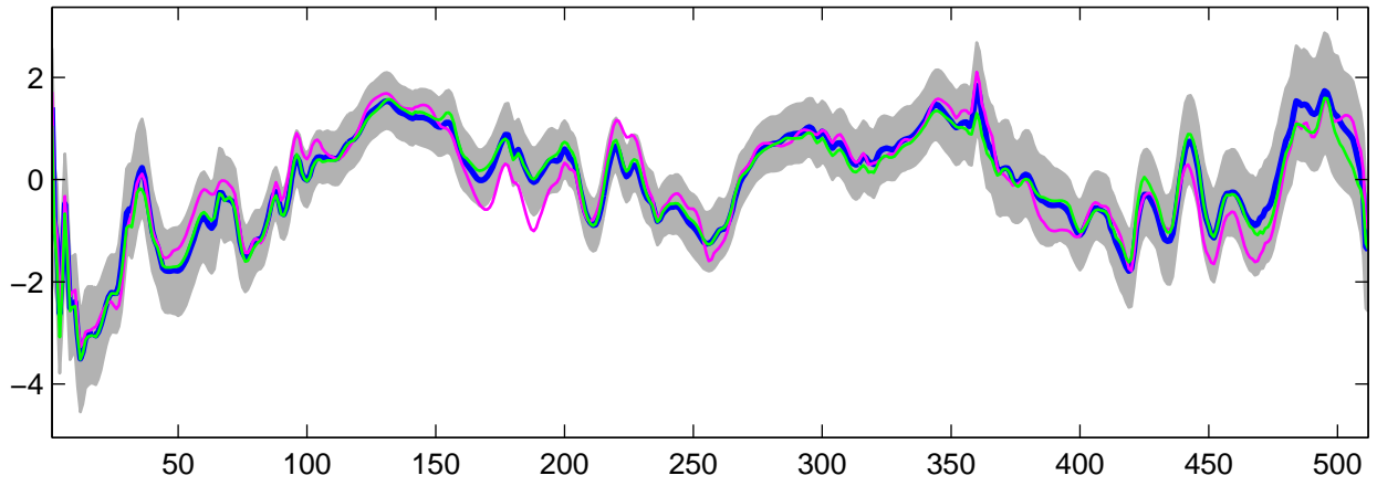
Estimated U_{16}(t) using G-WFMM: Normal data, run 5
