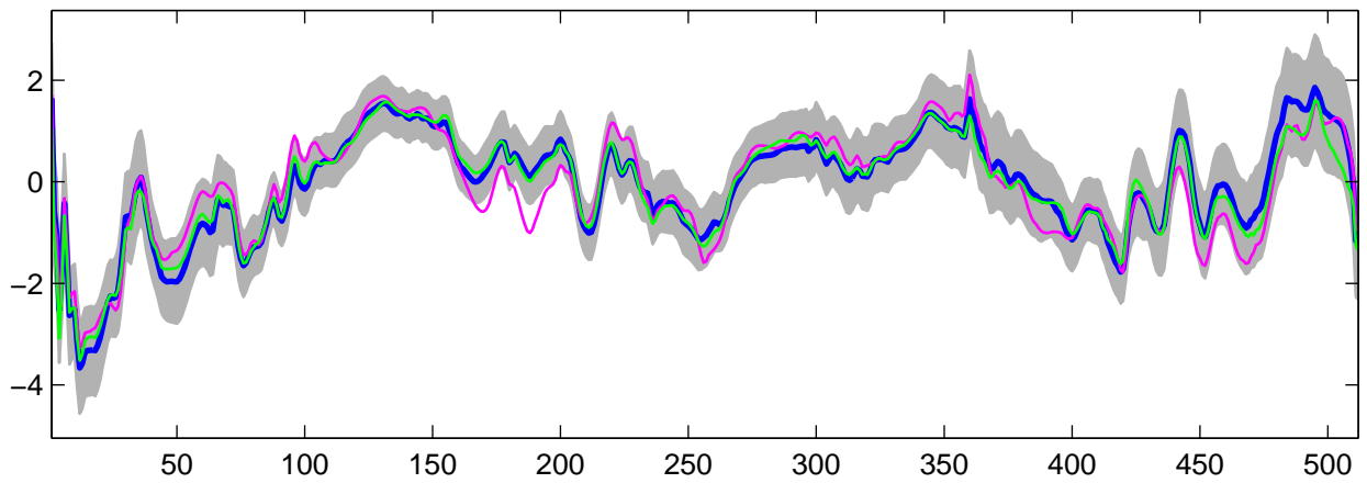
Estimated U_{16}(t) using R-WFMM: Normal data, run 5
