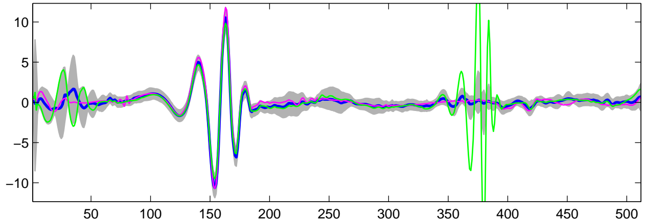
Estimated U_{16}(t) using G-WFMM: t_1 data, run 5
