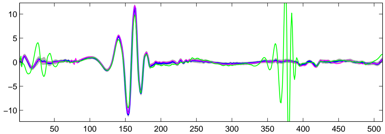
Estimated U_{16}(t) using R-WFMM: t_1 data, run 5
