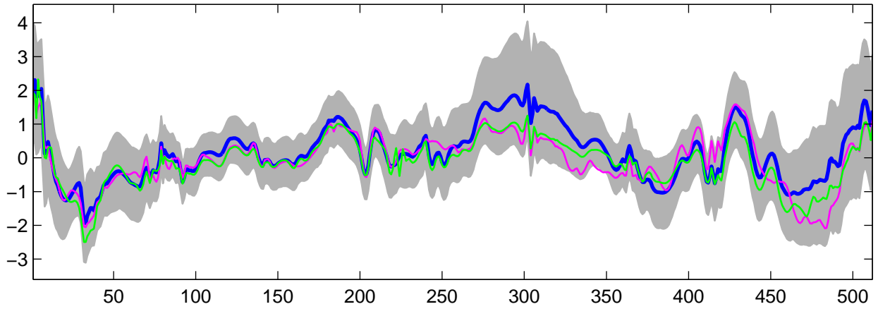
Estimated U_{16}(t) using G-WFMM: t_2 data, run 5
