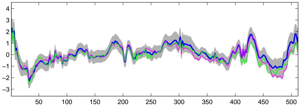
Estimated U_{16}(t) using R-WFMM: t_2 data, run 5
