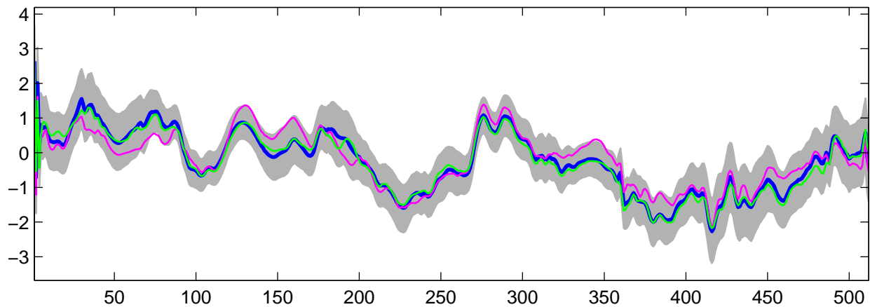
Estimated U_{16}(t) using G-WFMM: t_3 data, run 5
