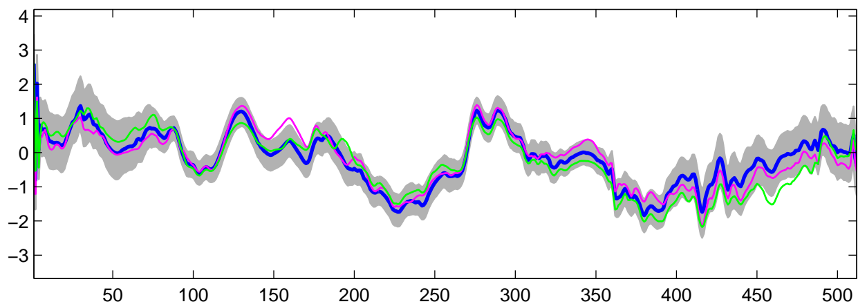
Estimated U_{16}(t) using R-WFMM: t_3 data, run 5
